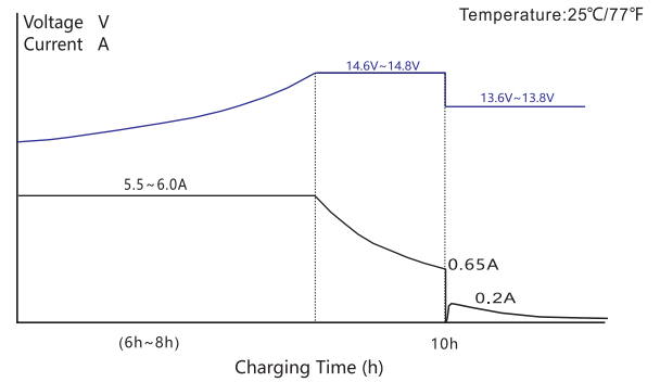
Charging Characteristics@25°C(77°F)
