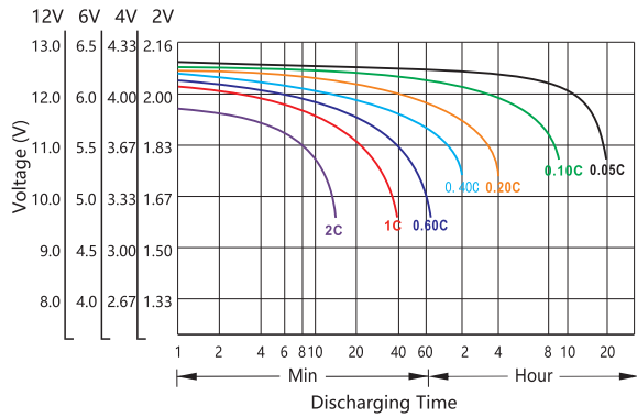
Discharging Characteristics@25°C(77°F)
